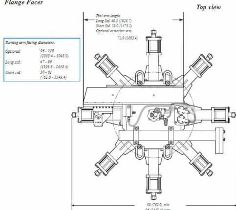
Standard ID-Mount Flange Facer
