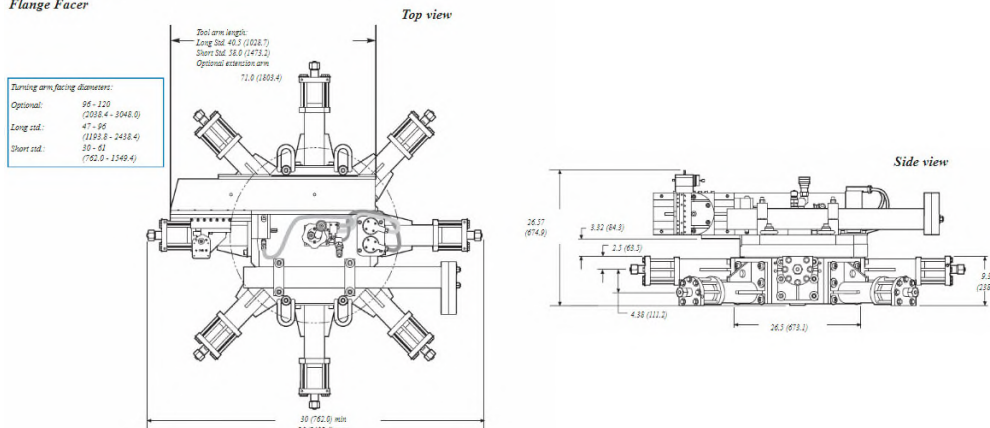
Standard ID-Mount Flange Facer
