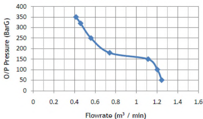
Triplex Pump 1 Performance (@ 2100 revs and Hydraulic Pressure 4,440 psi)
